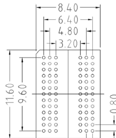
PCB PATTERN (Top View)
